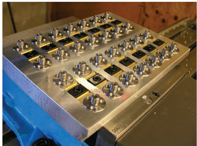
Fixtured with Mitee-Bite Machinable Uniforce® Clamps
