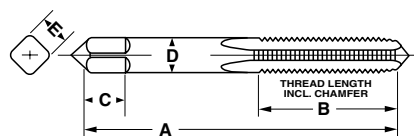
Size #0-12 Machine Screw Sizes 1.6-6.3mm
